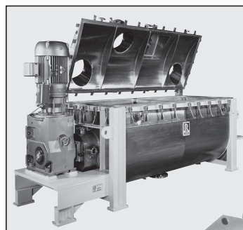
Space-saving drive designs are available, as on this 100 cu.ft., 40 HP sanitary vacuum dryer.
