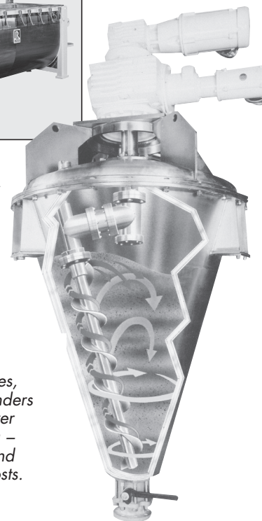
Space-saving drive designs are available, as on this 100 cu.ft., 40 HP sanitary vacuum dryer.
