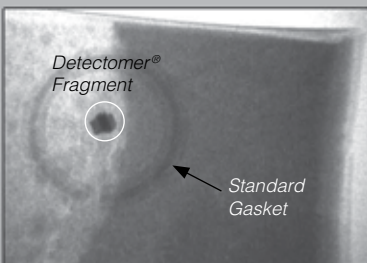
Box of Corn Muffin Mix X-ray
